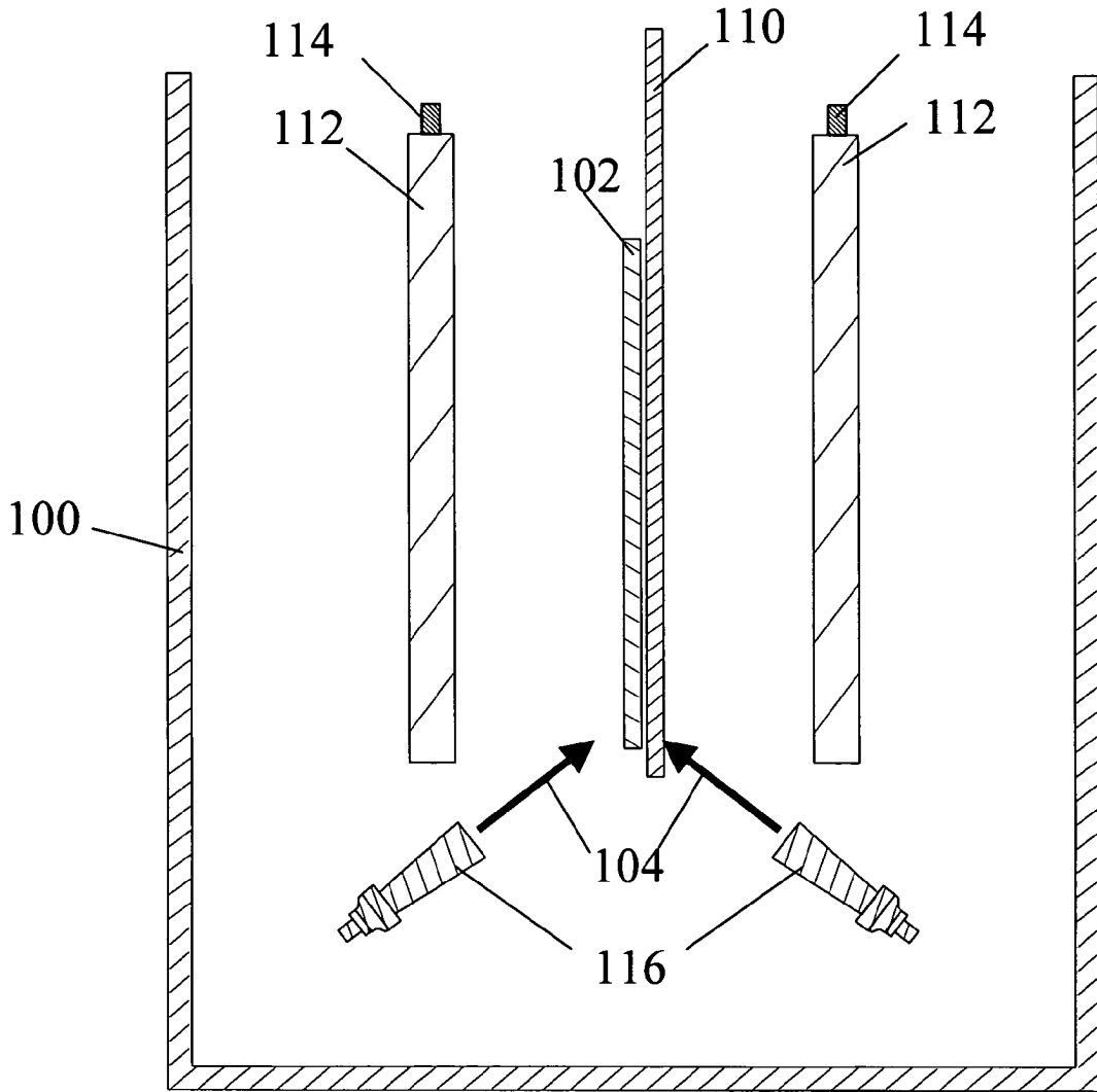
FIG. 5 PRIOR ART
