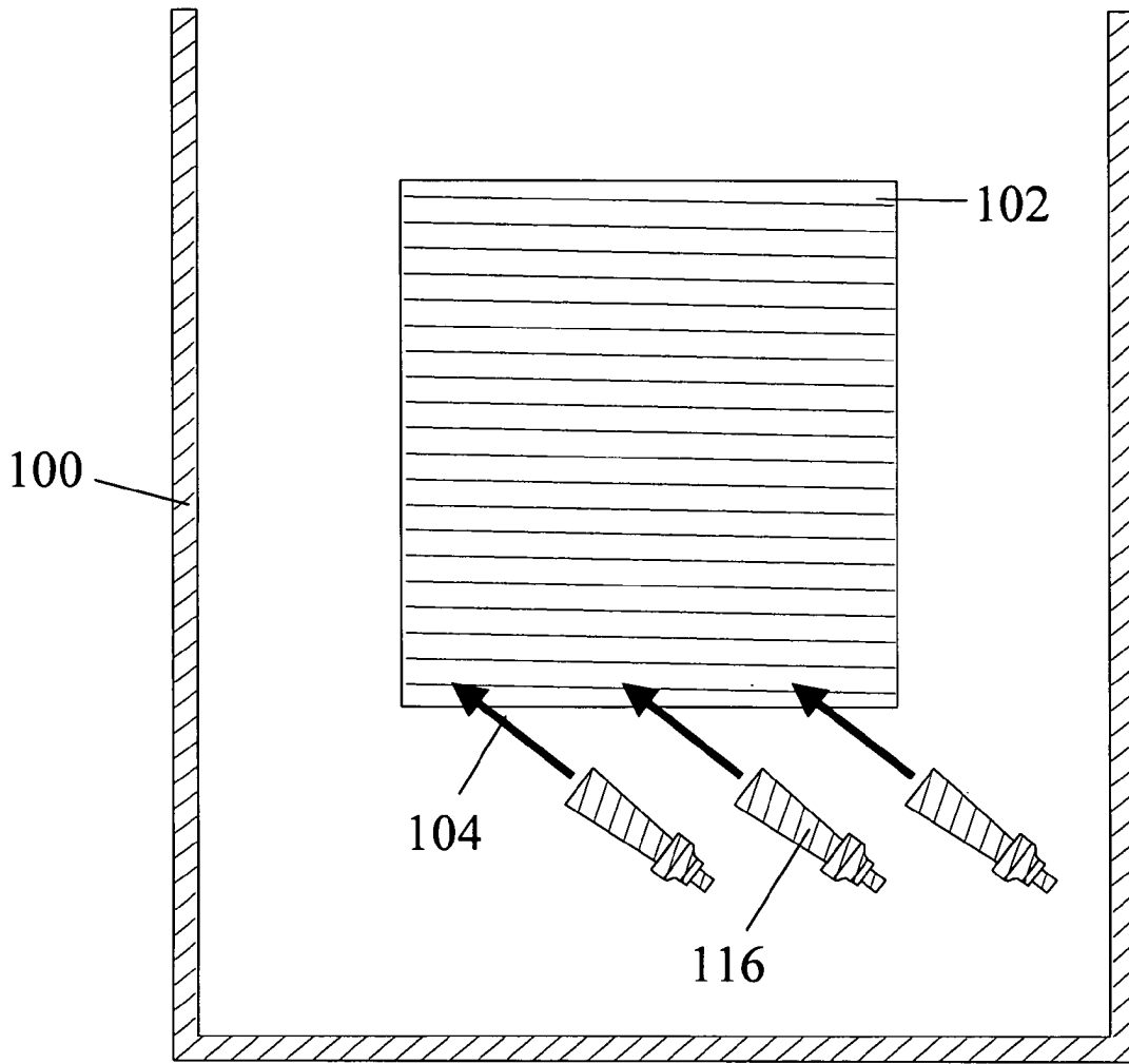
FIG. 7 PRIOR ART
