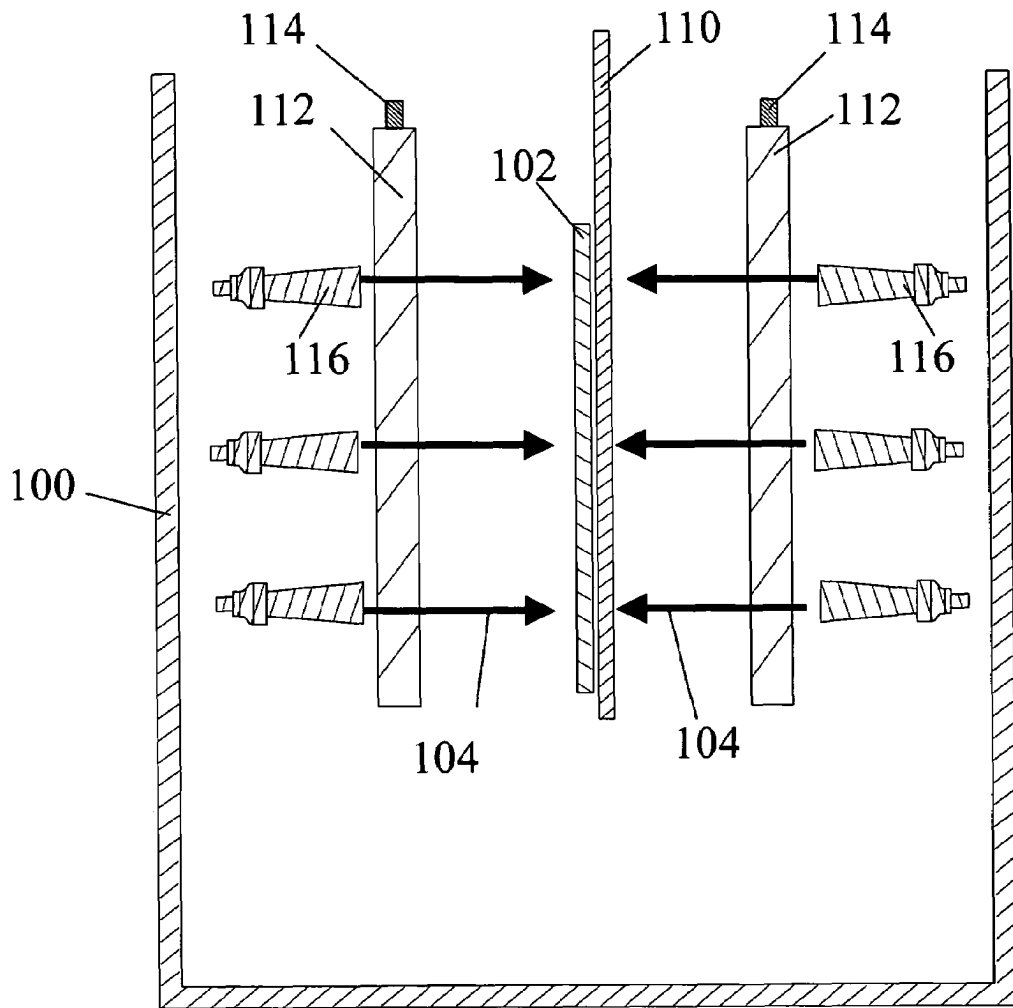
FIG. 3 PRIOR ART
